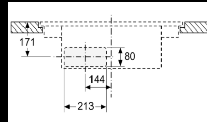
Unit Cut-Out Plano (From front view)
