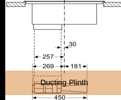
Unit Cut-Out Plano (From front view)
