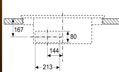
Unit Cut-Out (From front view)
